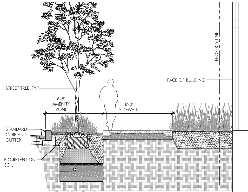
FLORIDA AVENUE - STREET SECTIONS SCALE: 3/16" = 1'-0"
