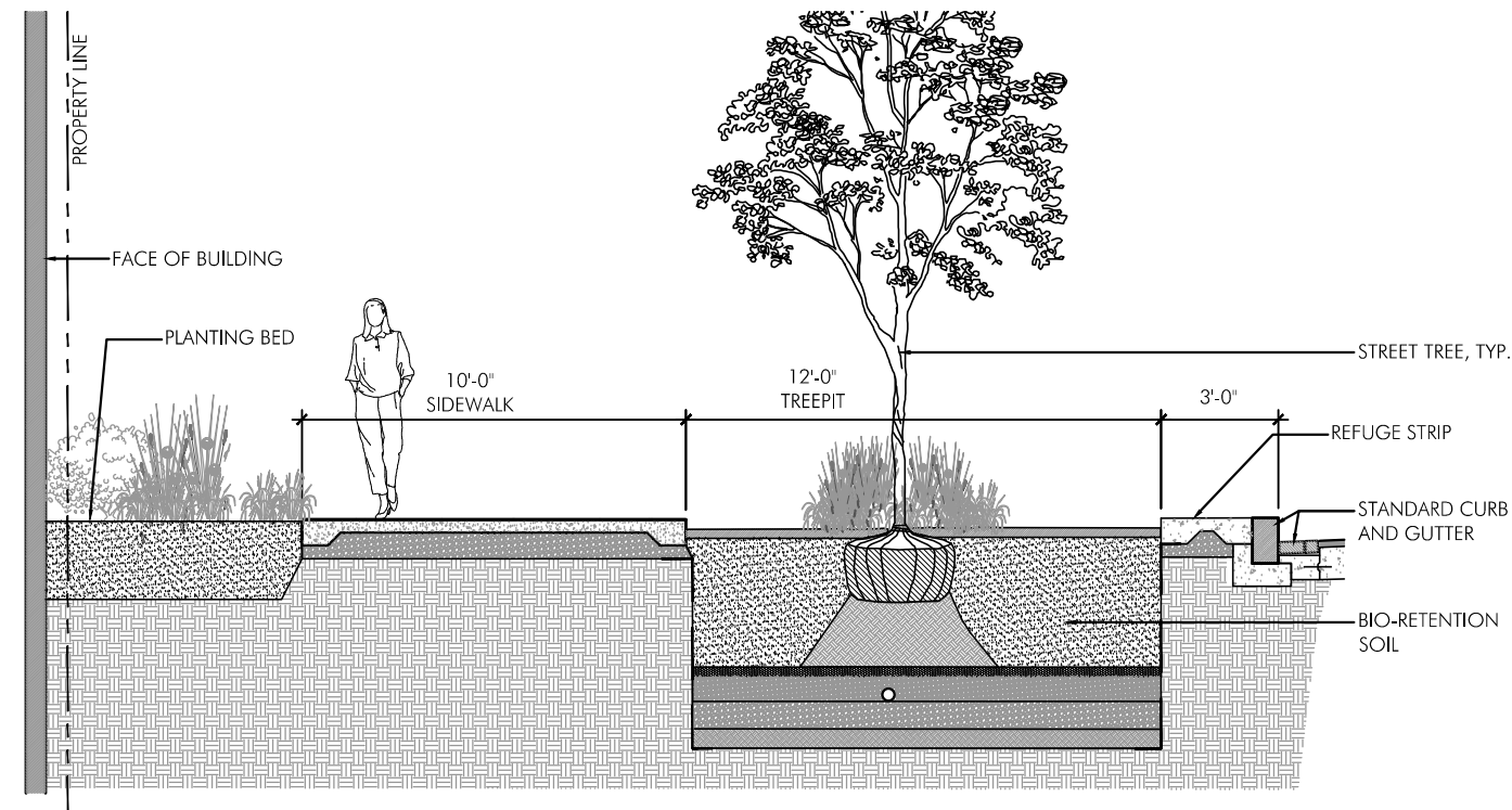
5TH STREET - STREET SECTIONS SCALE: 3/16" = 1'-0"
