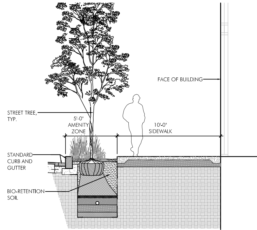
4TH STREET - STREET SECTIONS SCALE: 3/16" = 1'-0"
